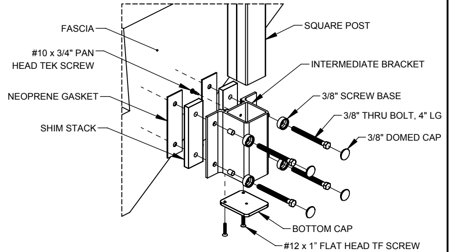
② TYP. POST TO DECK CONNECTION SCALE 1 : 8
