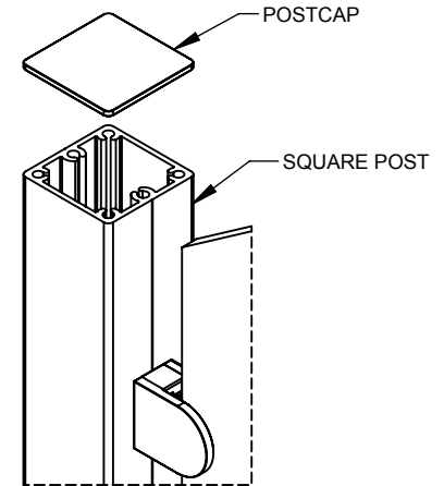
② TYP. POSTCAP TO SQUARE POST SCALE 1 : 4
