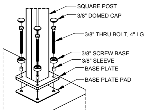
3 TYP. DECK MOUNTING CONNECTION SCALE 1 : 8
