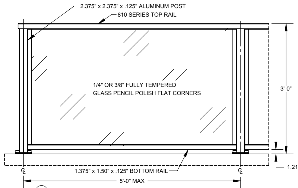
1 GLASS WITH TOP & BOTTOM RAIL, DECK MOUNT
