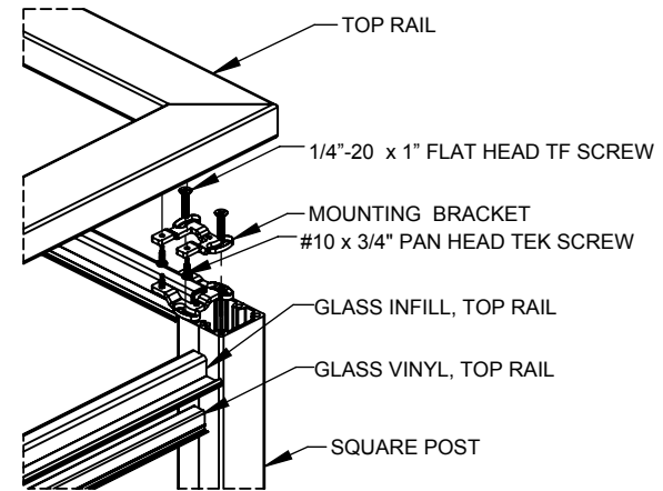
6 TYP. CORNER CONNECTION
