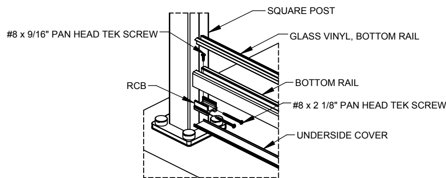
4 TYP. BOTTOM RAIL CONNECTION SCALE 1 : 8
