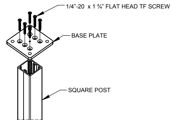
2 TYP. BASE PLATE TO POST CONNECTION SCALE 1 : 8
