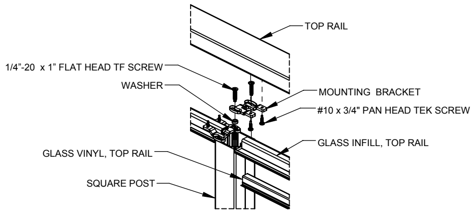
5 TYP. TOP RAIL CONNECTION
